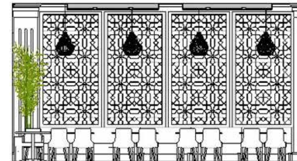
① Restaurant Bench View 1/4" = 1'-0"
