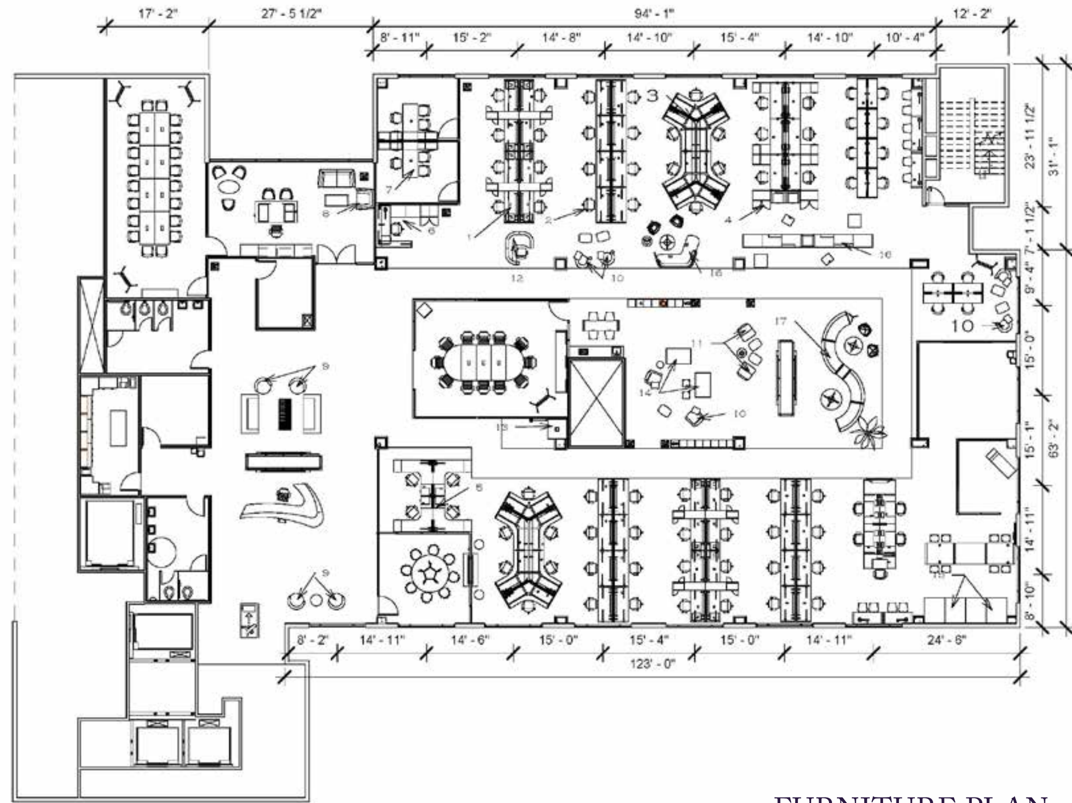
FURNITURE PLAN
