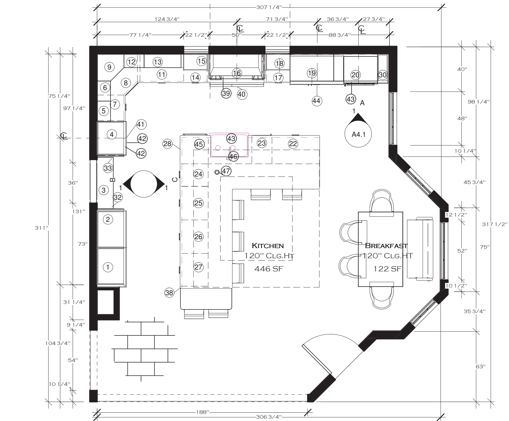
① First Floor Plan 1/4" = 1'-0"
