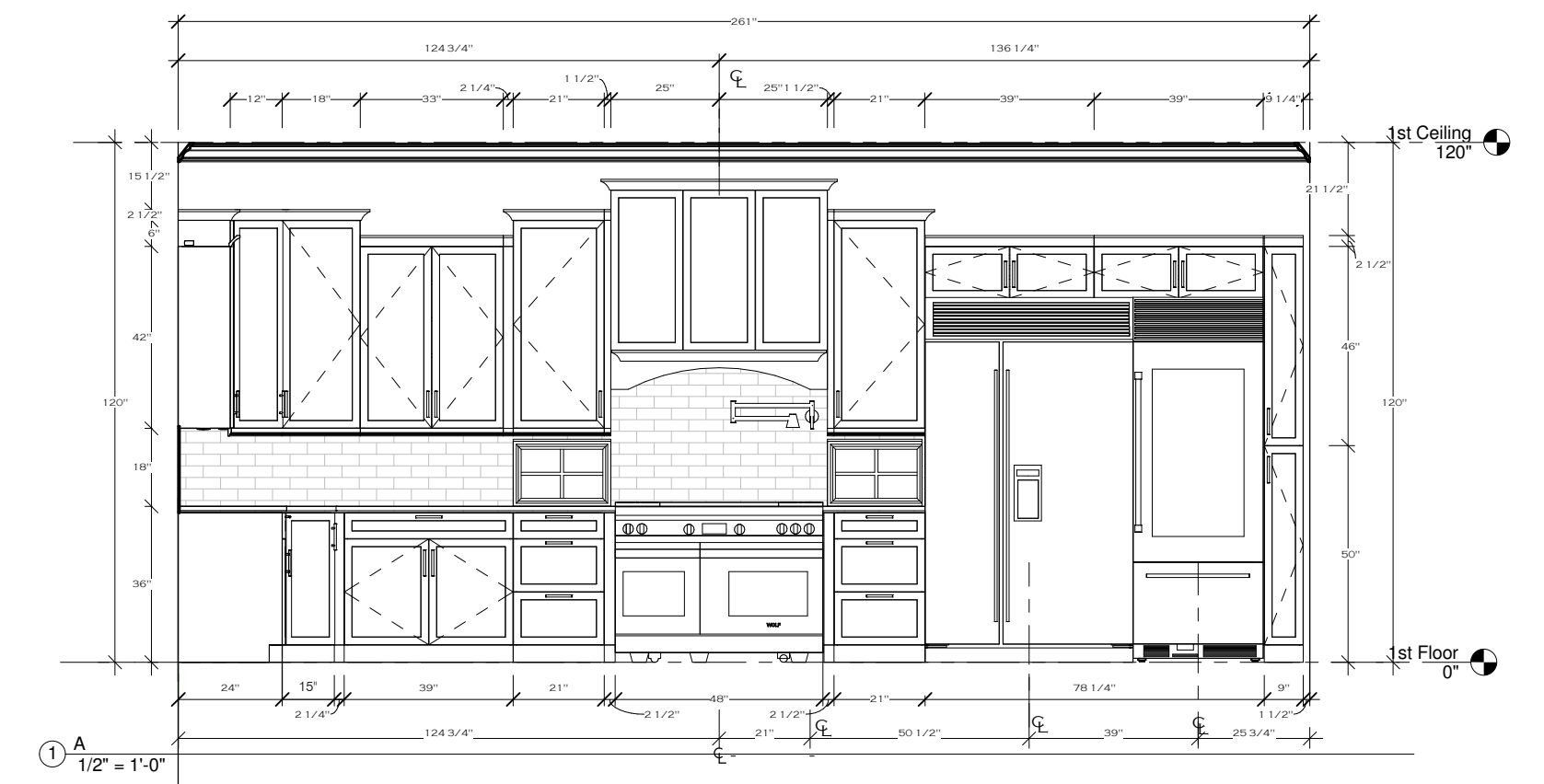
KITCHEN -ELEVATIONS
